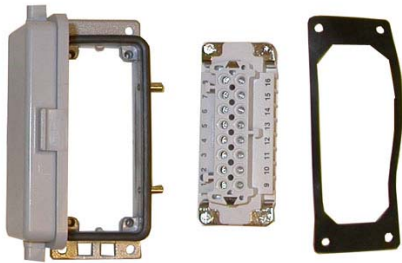
For DC Caster installations only 809926 Mating connector kit 16p, for SLS (bulkhead, only for connector beams)
